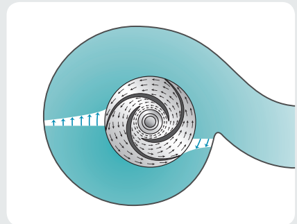
Flygt hydraulic design reduces slurry velocity
