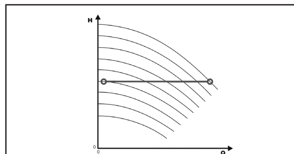
Control for constant pressure
