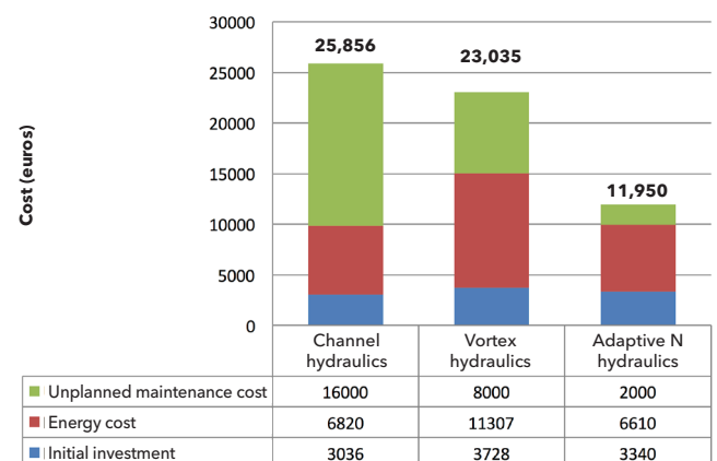
Figure 15: Simplified LCC analysis based on operation time 12 hours/day
