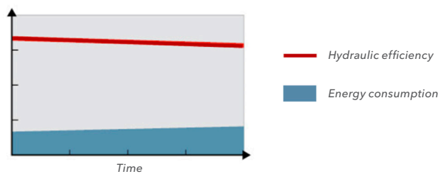
Figure 13c: Self-cleaning pump running continuously and intermittently
