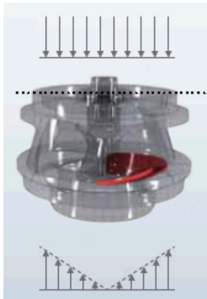
Figure 10: Force distribution during normal operation
